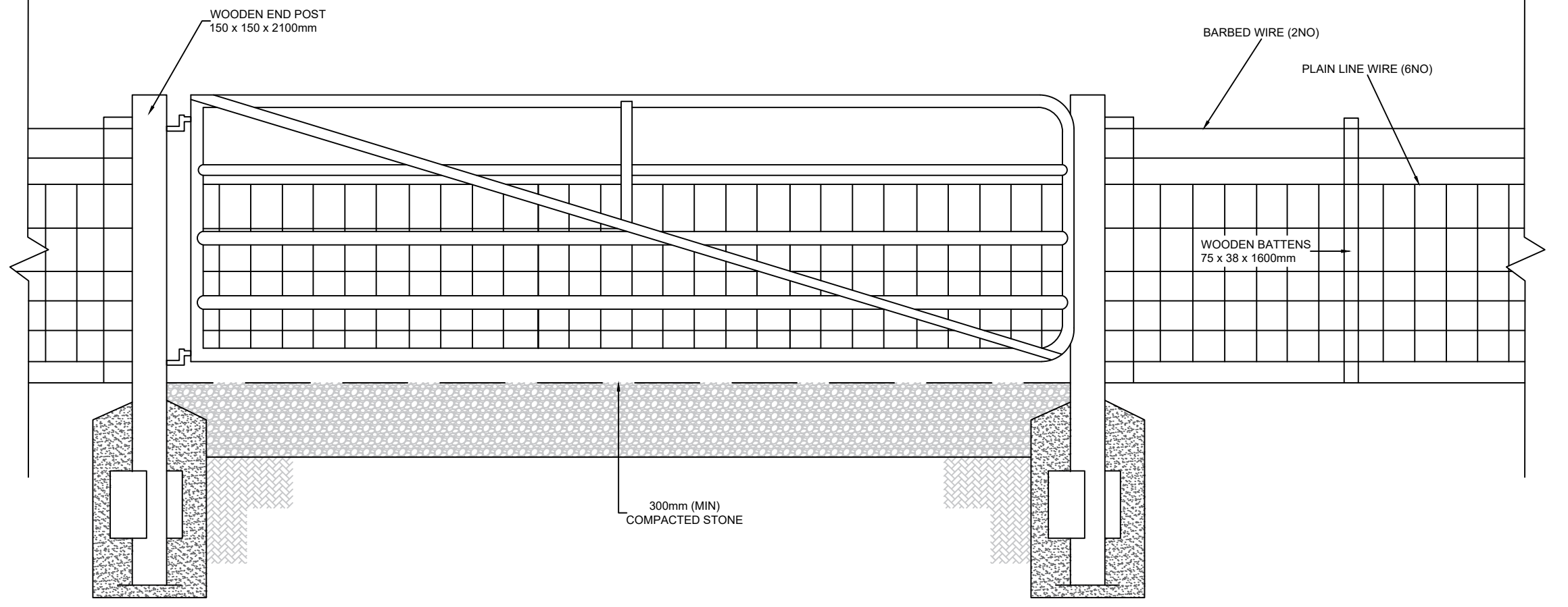
TYPICAL FENCE
